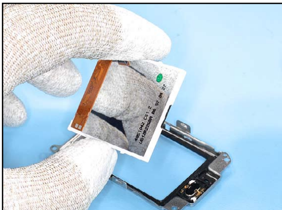
18. The LCD can be removed easily if both hooks are unlocked correctly.
